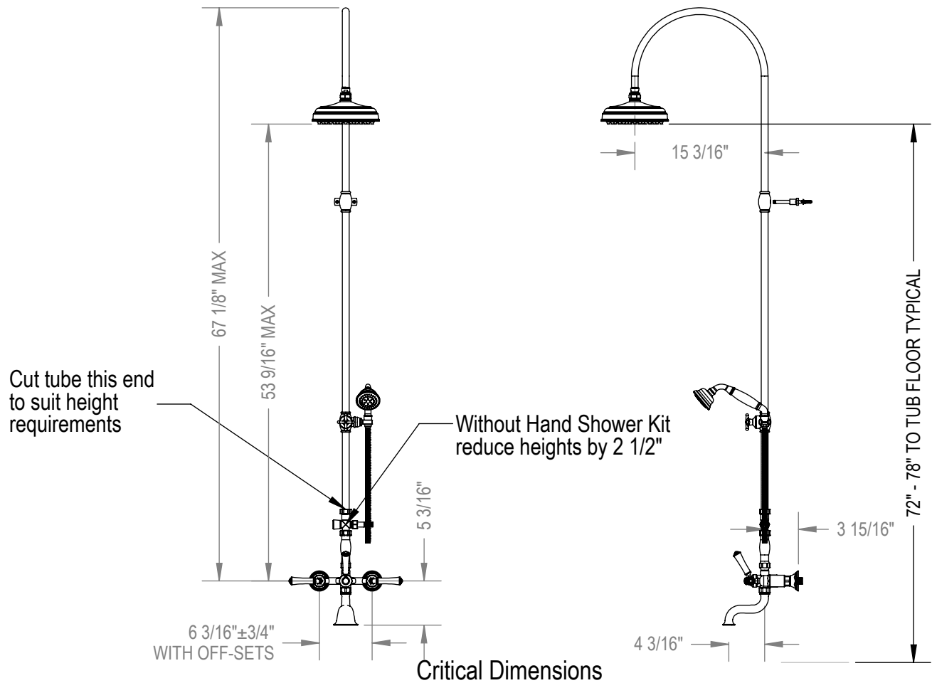
Wall Mount Tub & Shower w ith Optional Hand Held Shower Model: 2WRBRVL XX-XX
