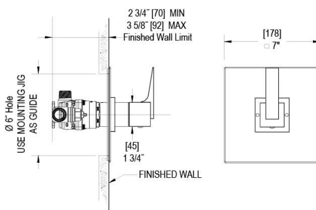
Pressure Balance Shower Valve Only with Stops
